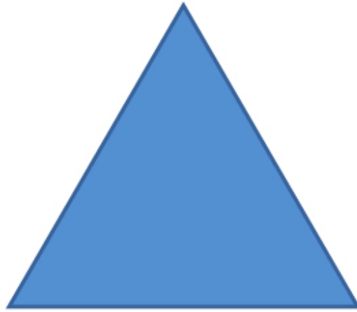
equilateral triangle
