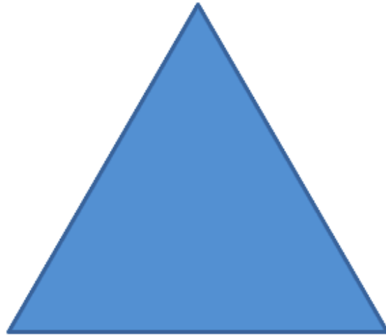
triangle
