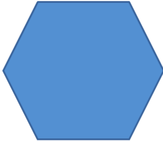
hexagon
