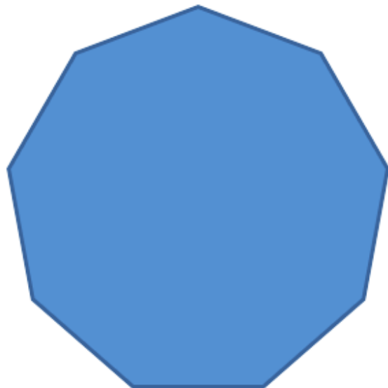
nonagon
