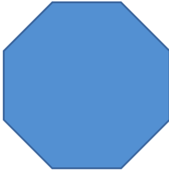
octagon
