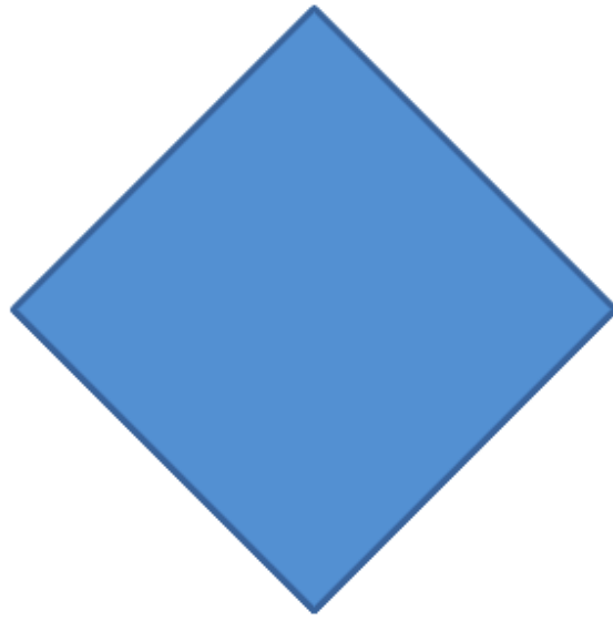
diamond
