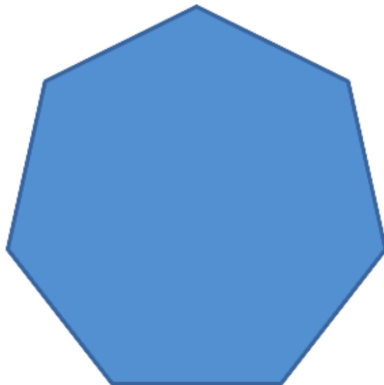
heptagon
