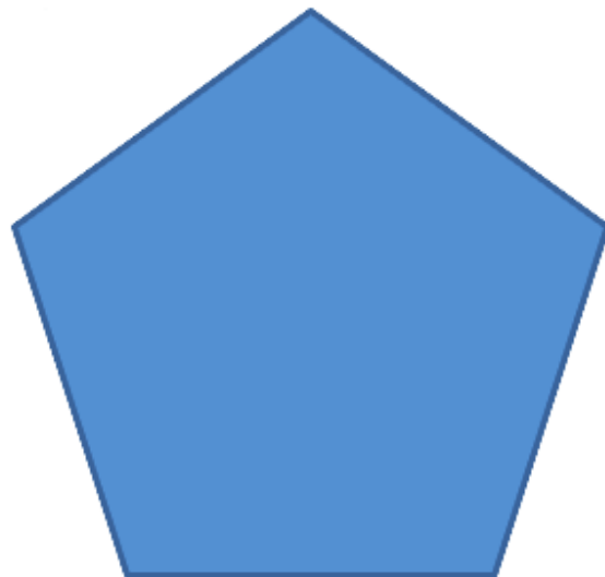
pentagon
