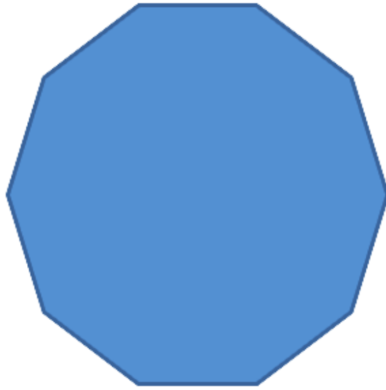
decagon
